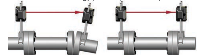
Dual-Fan™ Technology (2 lasers, 1 direction)
