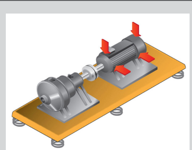
Duo-View™ live move screen shows live motor graphics of both alignment planes.
