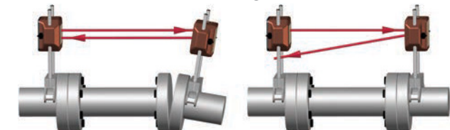
Dual-Fan™ Technology (2 lasers, 1 direction)
